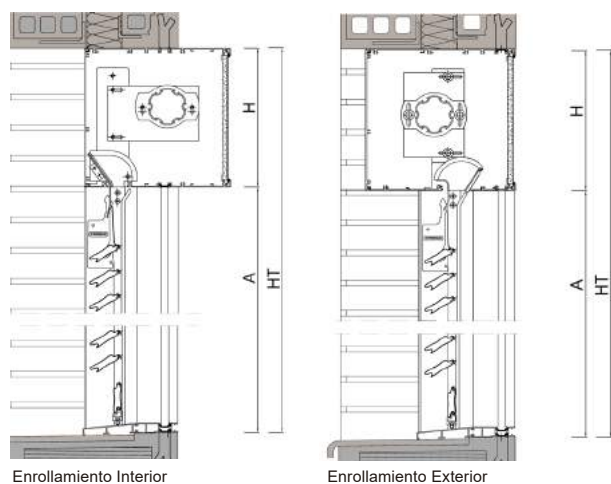
Enrollamiento Interior
